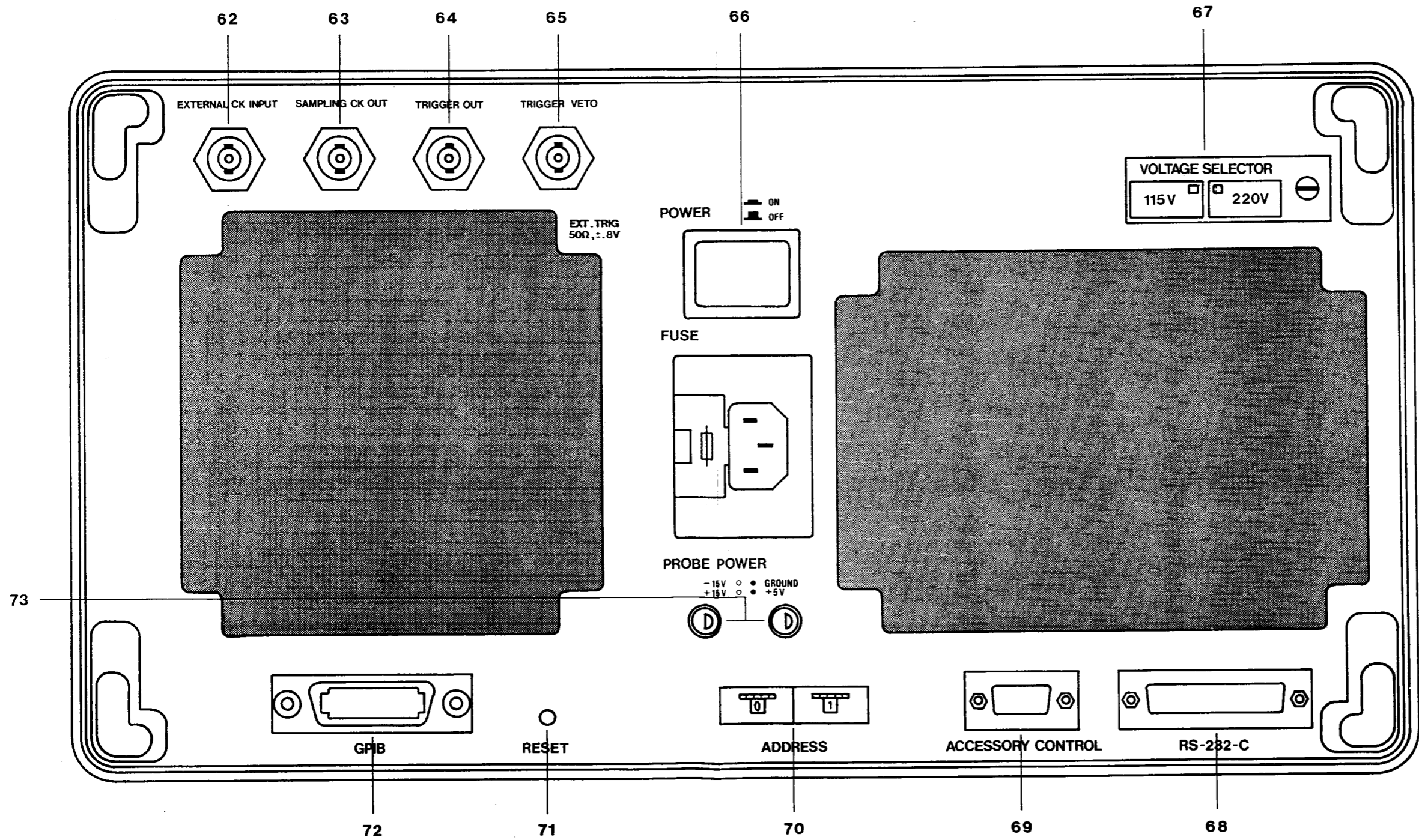
Figure 3: 9424 Rear Panel
